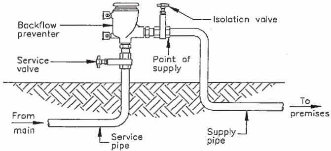
Example 8 – Unmetered supply with vacuum breaker backflow preventer
